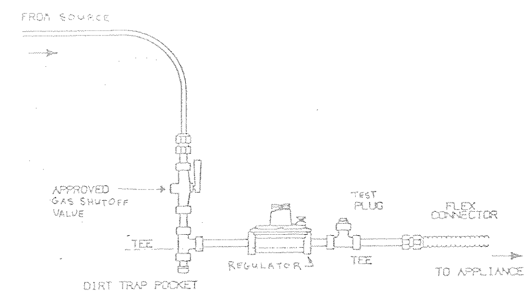
TYPICAL GAS CONNECTION DETAIL NO SCALE
