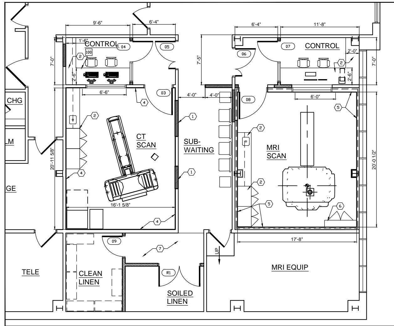
1 NEW FLOOR PLAN Scale: 1/4" = 1'-0"
