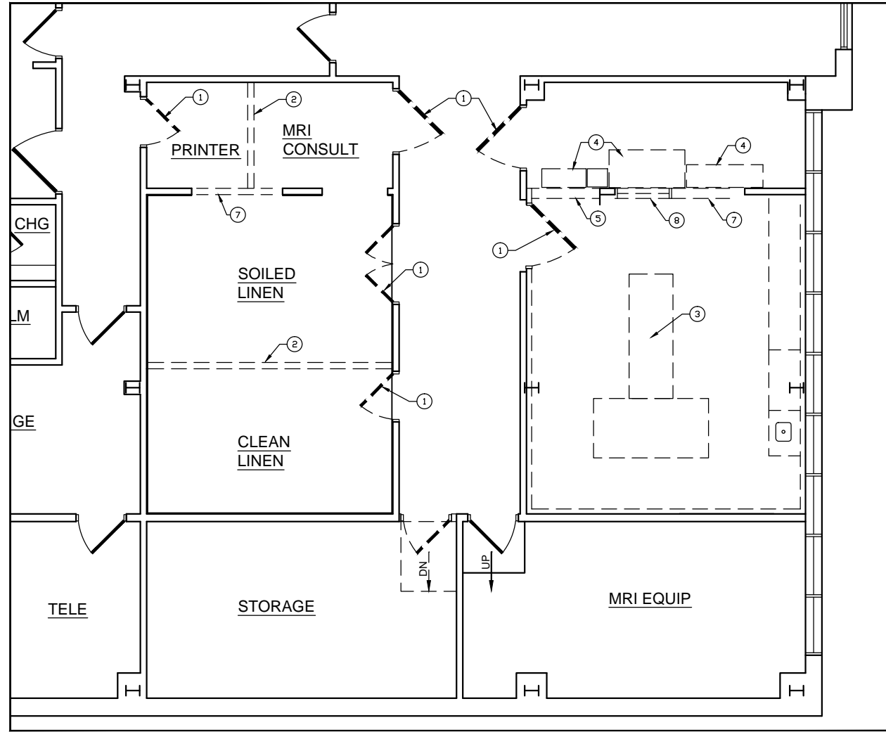
1 DEMOLITION PLAN Scale: 1/4" = 1'-0"
