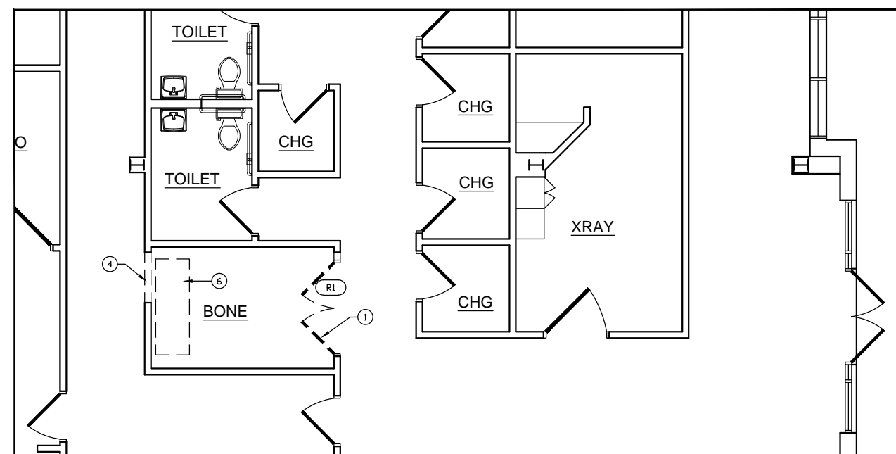
1 DEMOLITION PLAN Scale: 1/4" = 1'-0"
