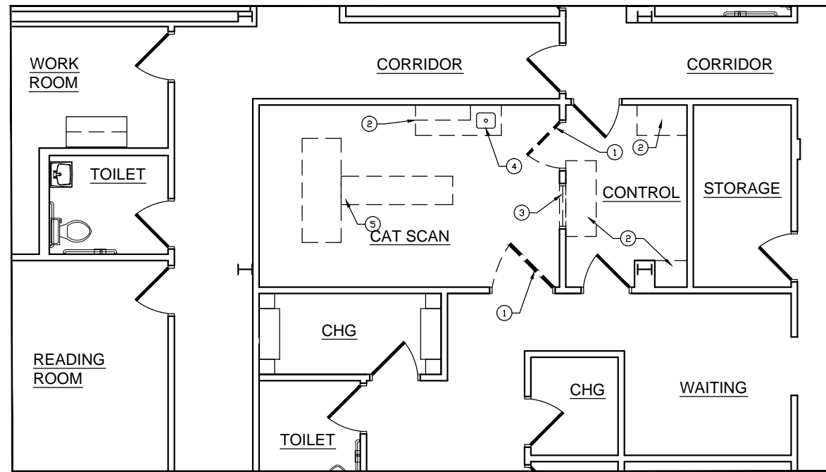
1 DEMOLITION PLAN Scale: 1/4" = 1'-0"
